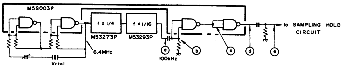
Fig. 4-5 Sampling pulse generator
