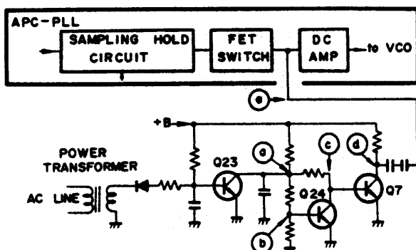
Fig. 4-11 Re-lock trigger circuit
