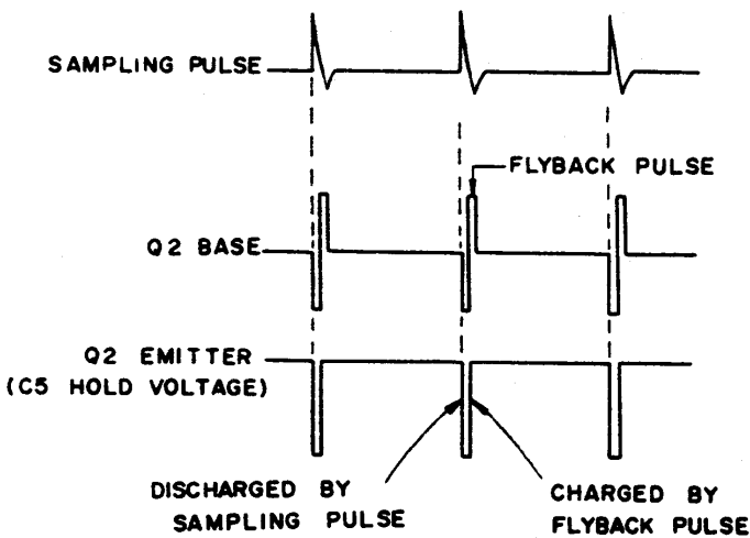
Fig. 4-7 Voltage waveforms
