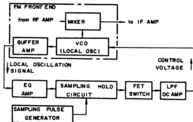
Fig. 4-3 Block diagram of APC circuit
