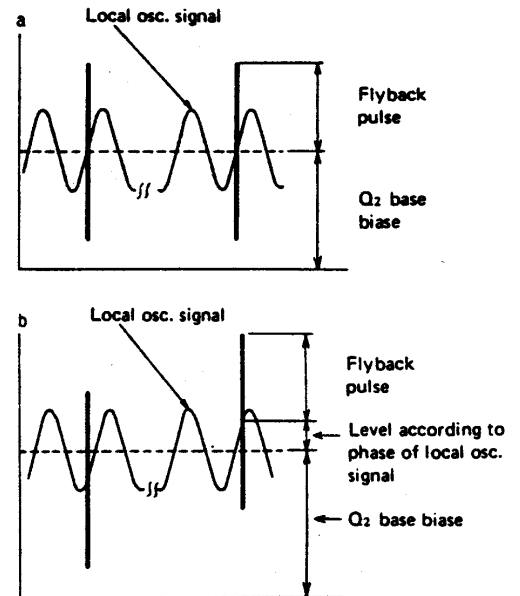
Fig. 4-8 Q_2 base waveforms
