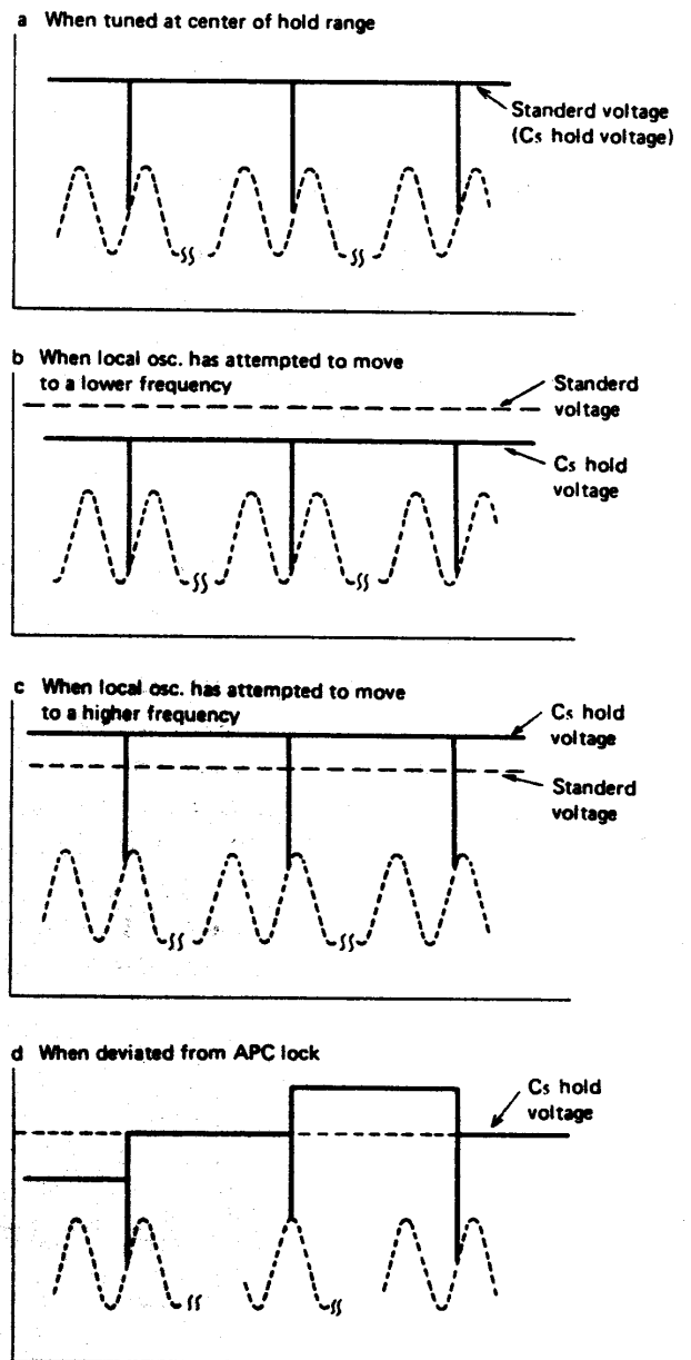
Fig. 4-9 C_5 hold voltage waveforms
