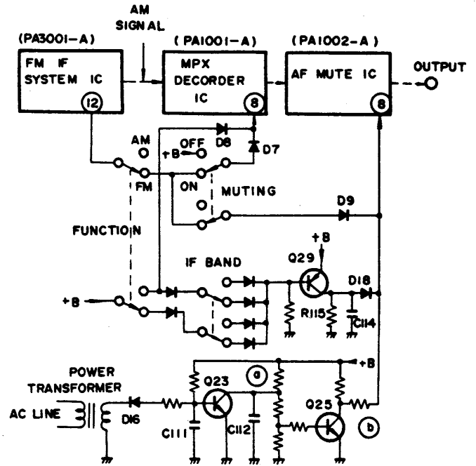
Fig. 4-13 Muting control circuit
