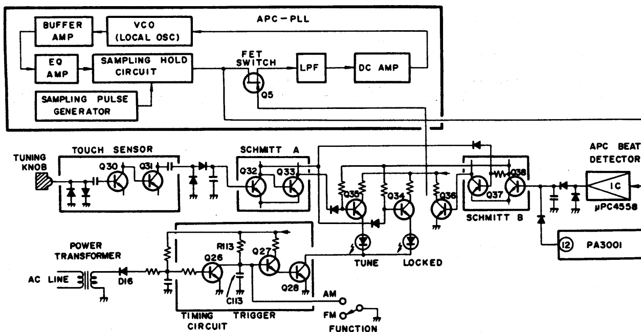
Fig. 4-10 APC operation control circuit
