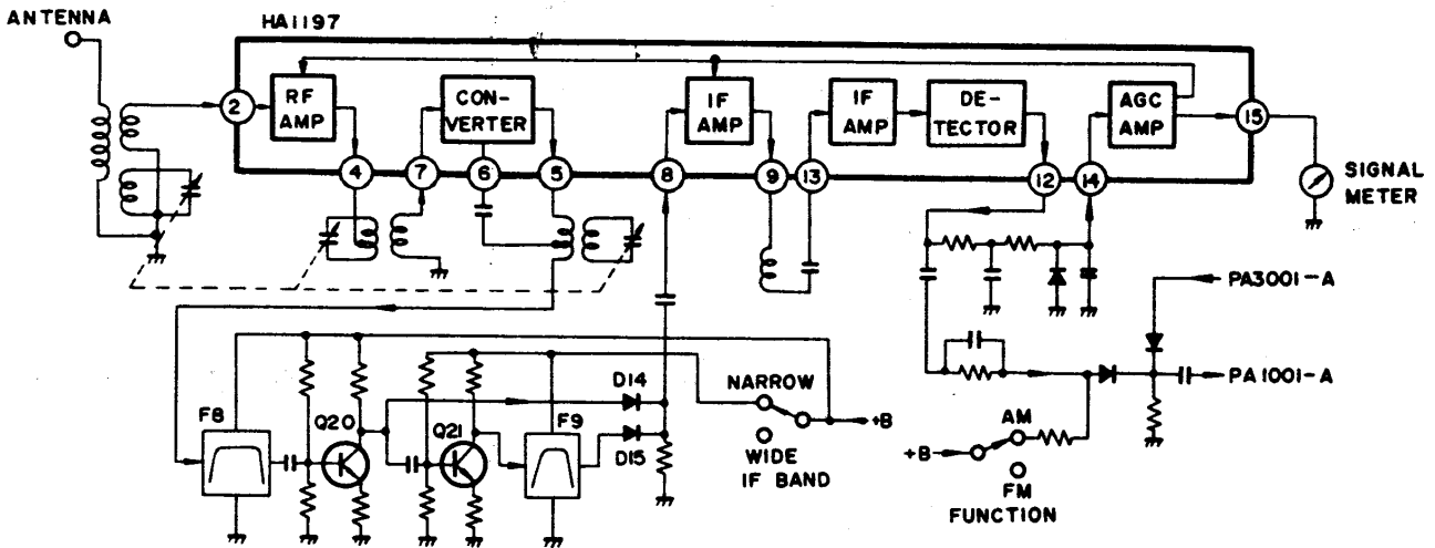
Fig. 4-15 AM tuner
