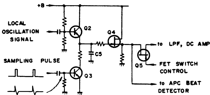
Fig. 4-6 Sampling hold circuit
