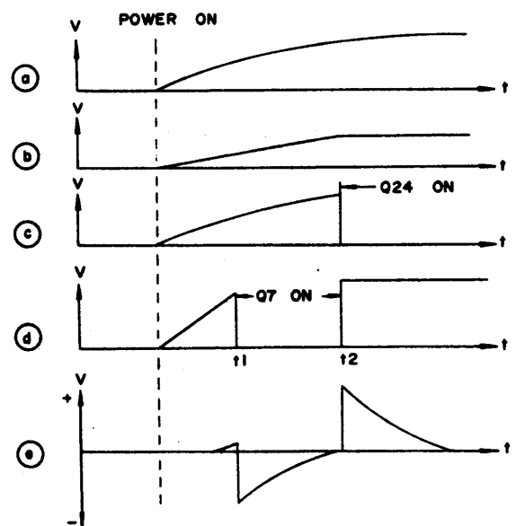
Fig. 4-12 Voltage waveforms
