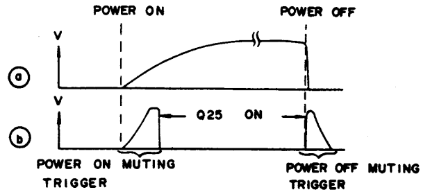
Fig. 4-14 Voltage waveforms
